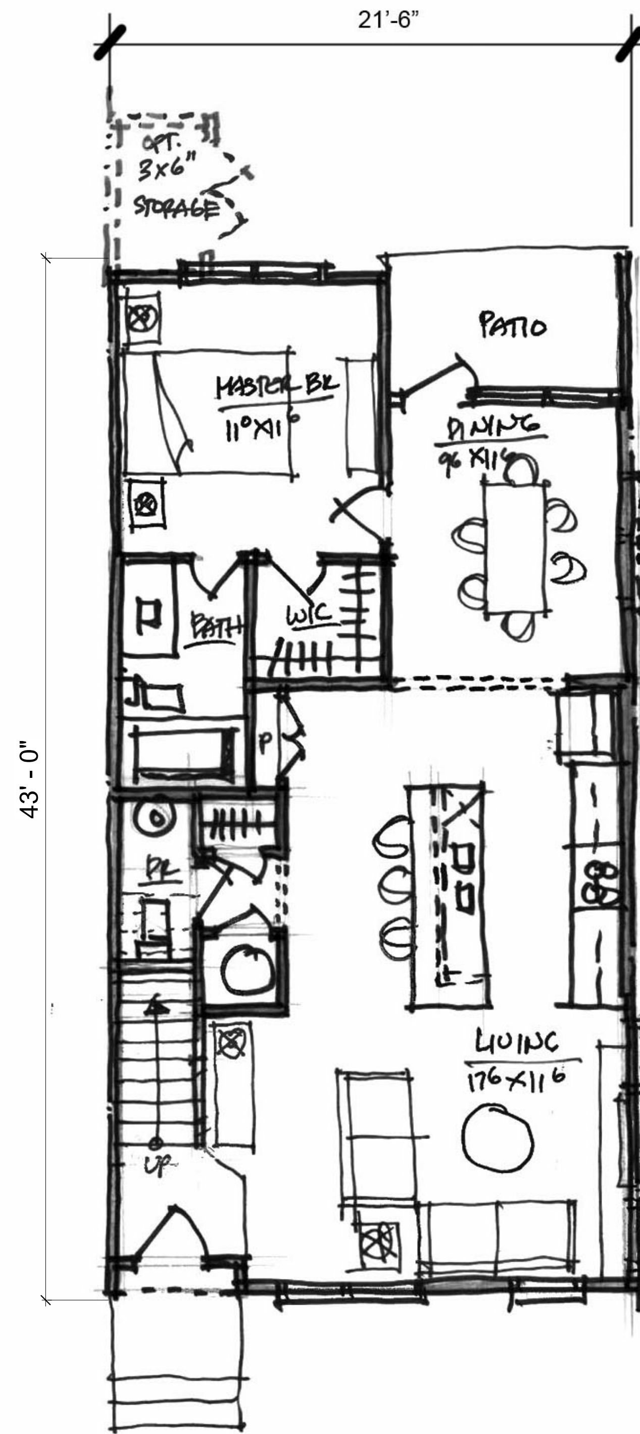
LOWER LEVEL PLAN ± 872 SF
